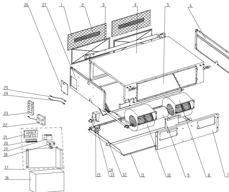
Model: GFH24K3CI exploded view and spare parts list.
