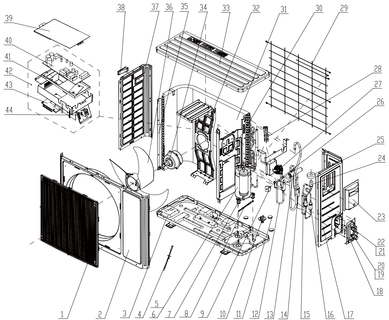
Model: GUHD18NK3C1O Exploded View and spare parts list:
