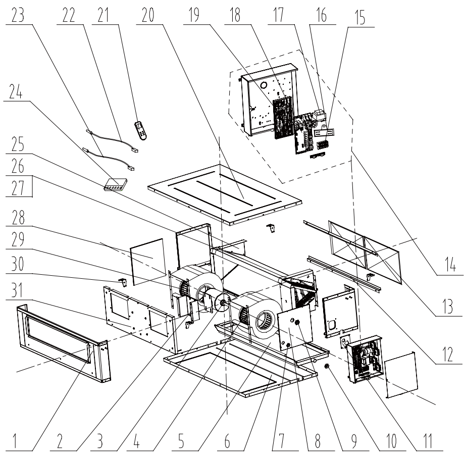
Model: GFH60K3CI exploded view and spare parts list.
