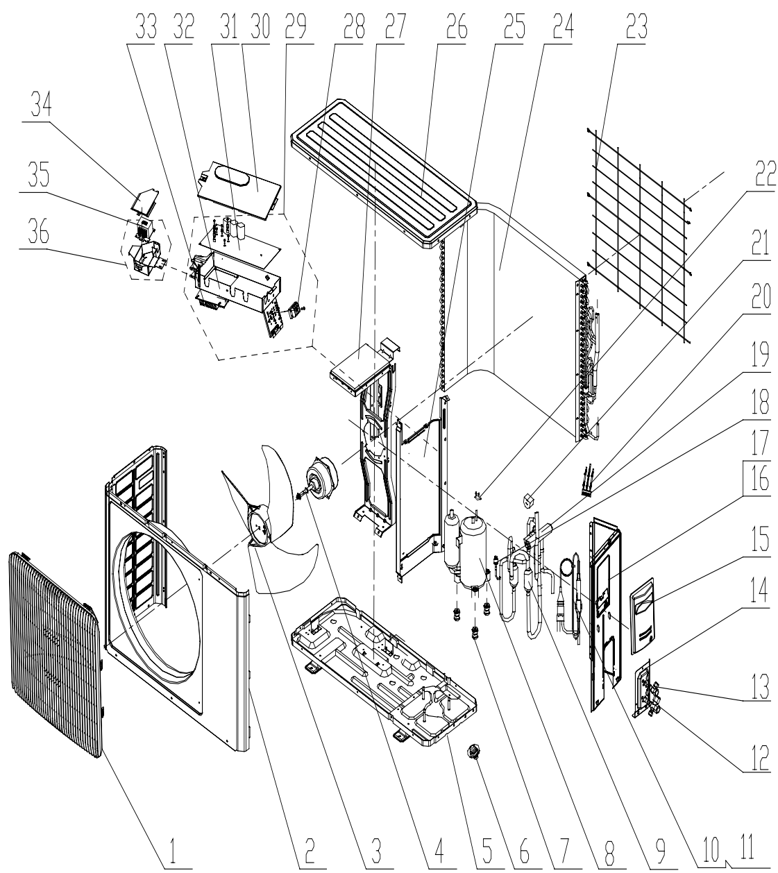
Model: GUHD09NK3C1O/GUHD12NK3C1O Exploded View and spare parts list:
