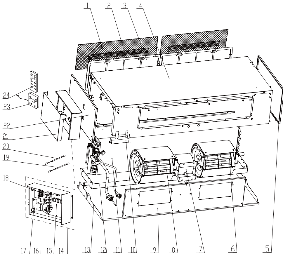
Model: GFH30K3CI exploded view and spare parts list.
