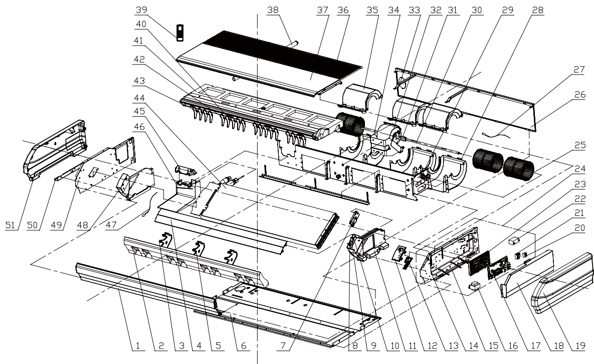
Model:GTH30K3CI exploded view and spare parts list.
