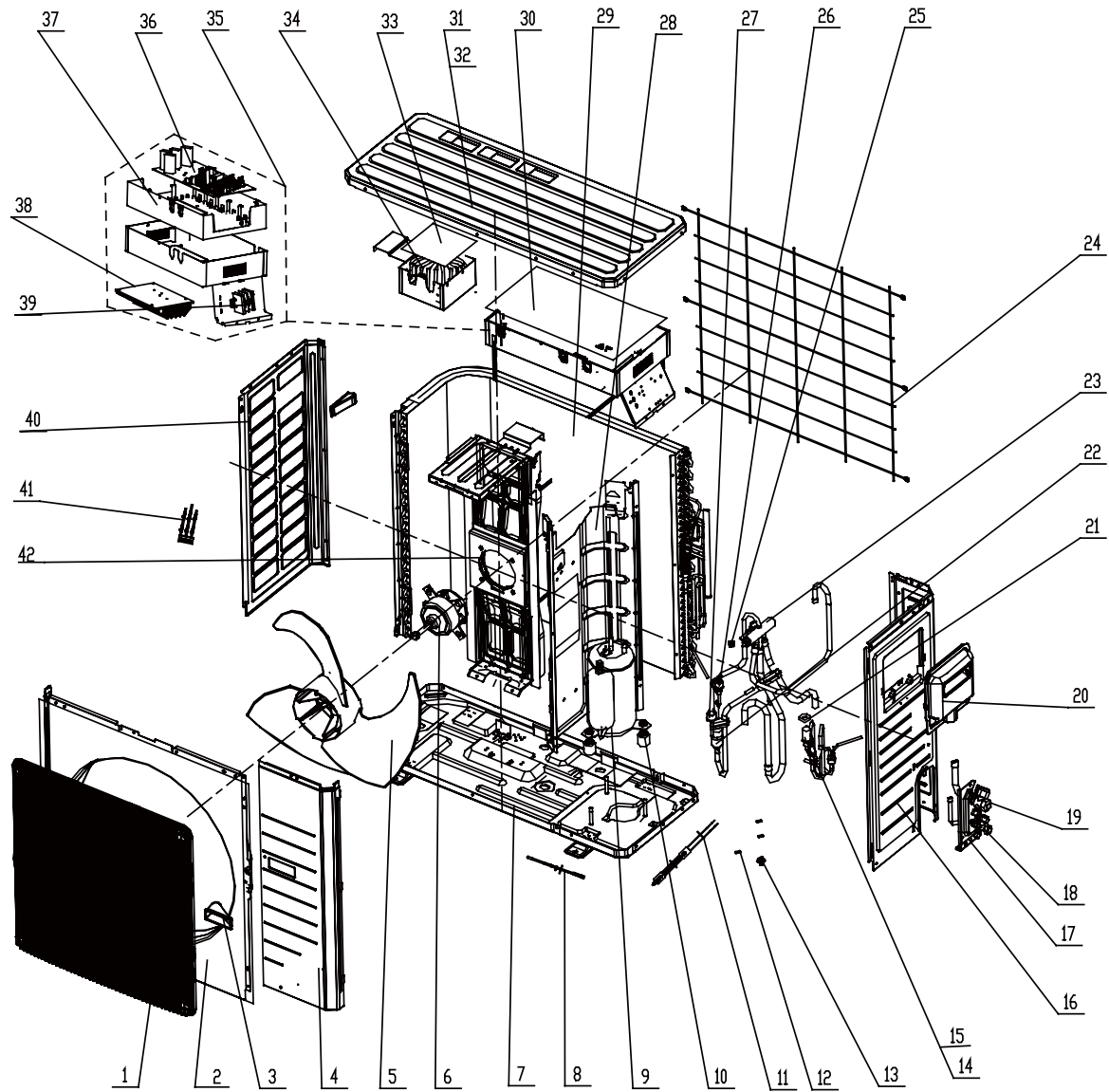
Model: GUHD24NK3C1O\GUHD30NK3C1O Exploded View and spare parts list
