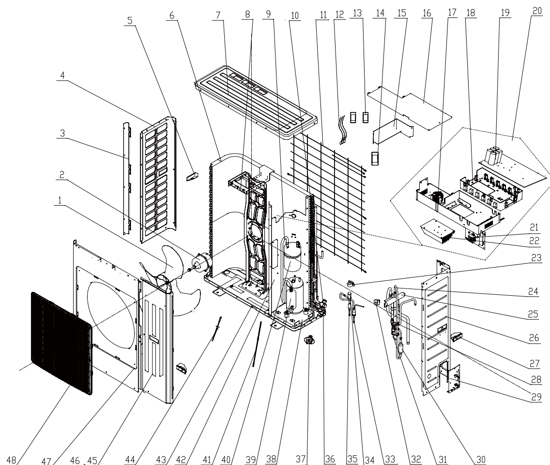
Model: GUHD36NK3C1O/GUHD42NK3C1O Exploded View and spare parts list
